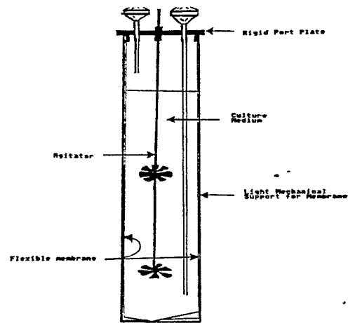
FIGURE 3 MECHANICAL AGITATOR FERMENTER
